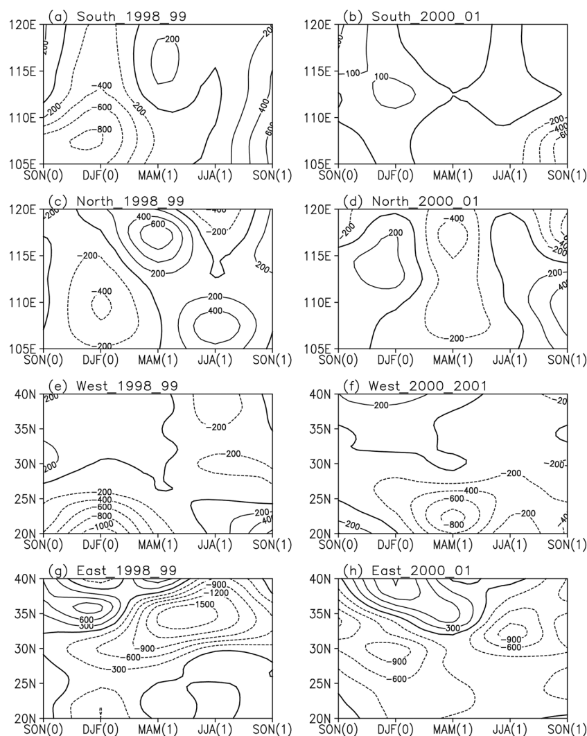
Figure 6. Anomalies of vertically integrated aerosol concentrations fluxes at the (a and b) south, (c and d) north, (e and f) west, and (g and h) east boundaries of eastern China from 1000 to 100 hPa during the La Niña events of (left) 1998/1999 and (right) 2000/2001.
