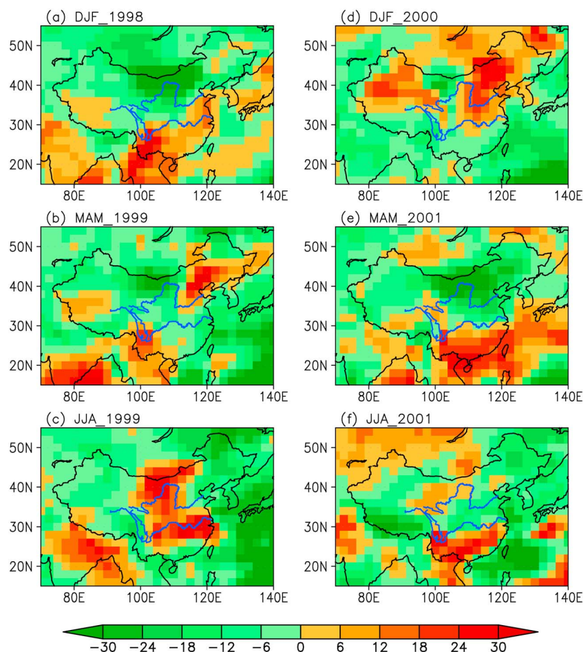
Figure 1. Spatial distribution of the surface-layer \text{PM}_{2.5} RPAD during the seasonal cycle for the La Niña Modoki events of (left) 1998/1999 and (right) 2000/2001.
