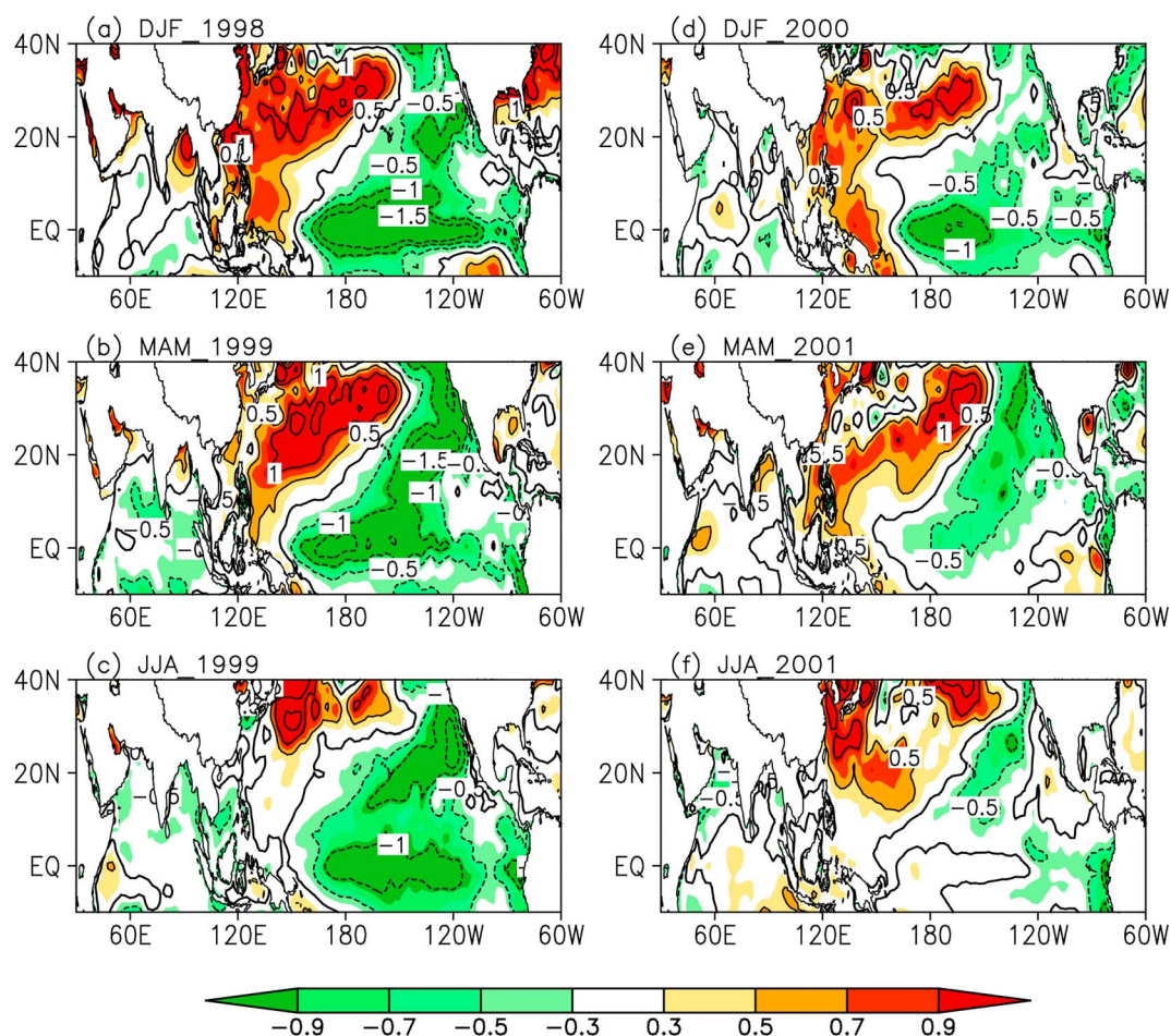
Figure 4. Horizontal distribution of SSTA (°C) based on the assimilated meteorological data during the La Niña Modoki events of (left) 1998/1999 and (right) 2000/2001.
